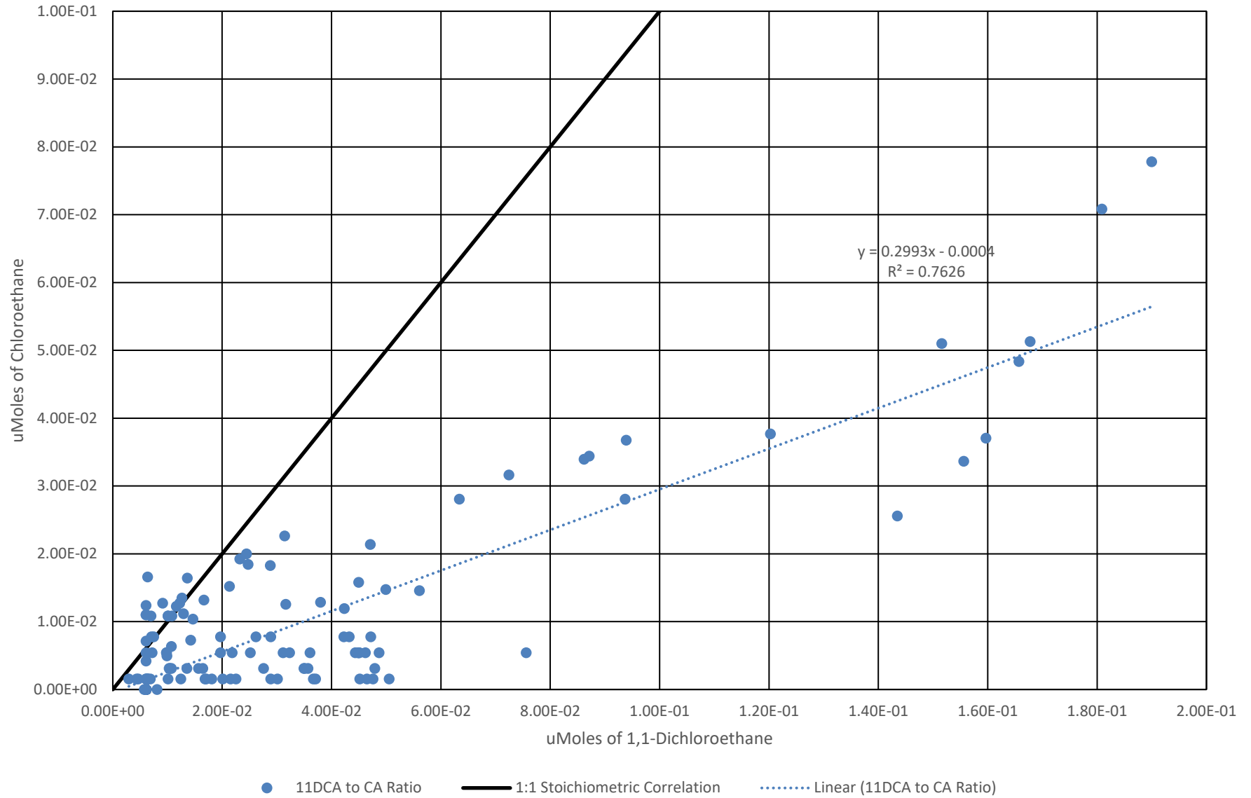
Chart 1 Closed Laurel Valley Center Sanitary Landfill, Permit No. 251 Sentinel and Performance Well 1,1-Dichloroethane to Chloroethane Ratios (2016-2020)
