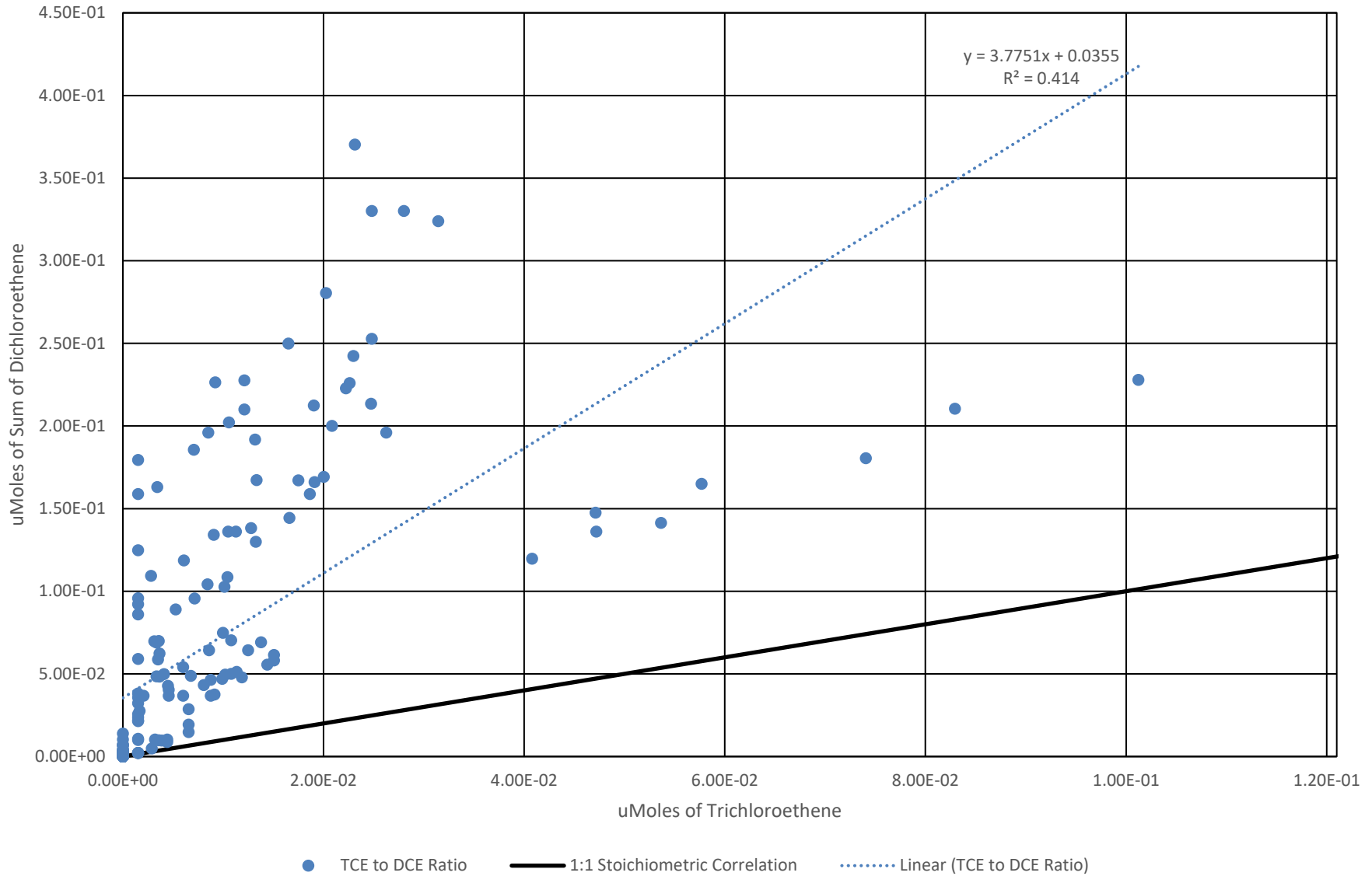
Chart 3 Closed Laurel Valley Center Sanitary Landfill, Permit No. 251 Sentinel and Performance Well Trichloroethene to Sum of Dichloroethene Ratios (2016-2020)
