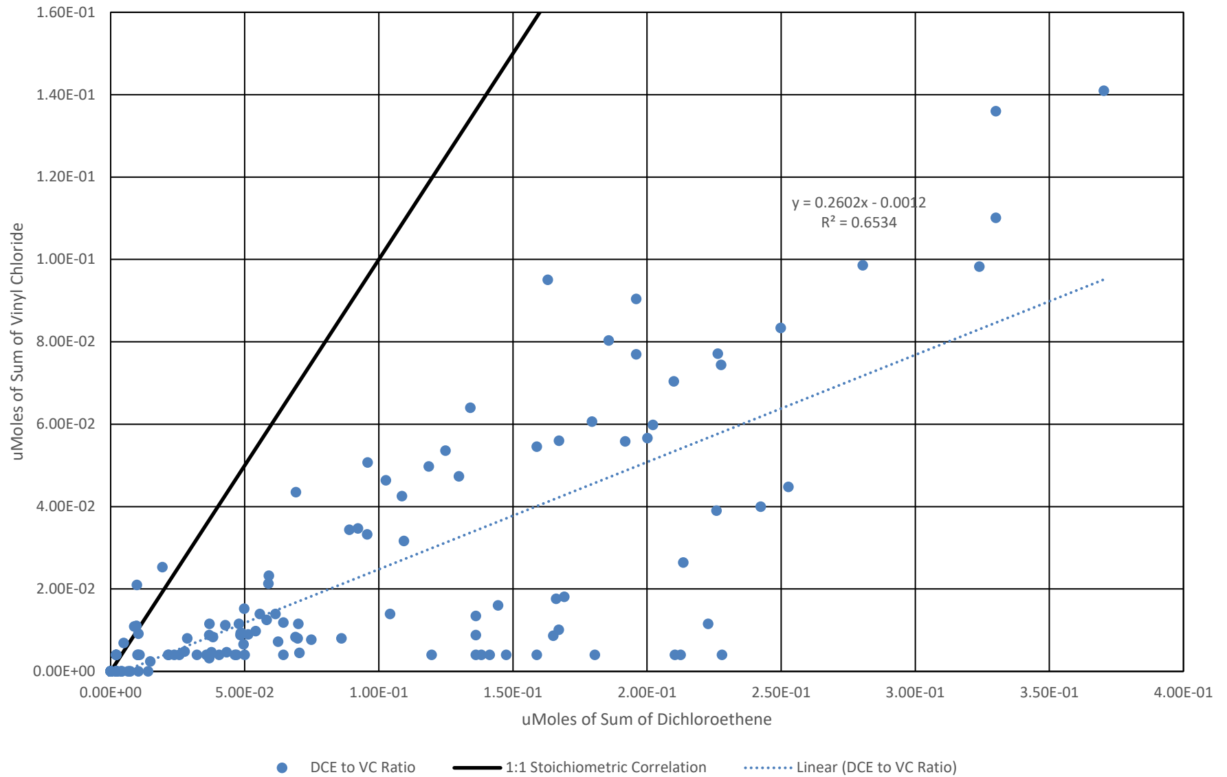
Chart 4 Closed Laurel Valley Center Sanitary Landfill, Permit No. 251 Sentinel and Performance Well Sum of Dichloroethene to Vinyl Chloride Ratios (2016-2020)
